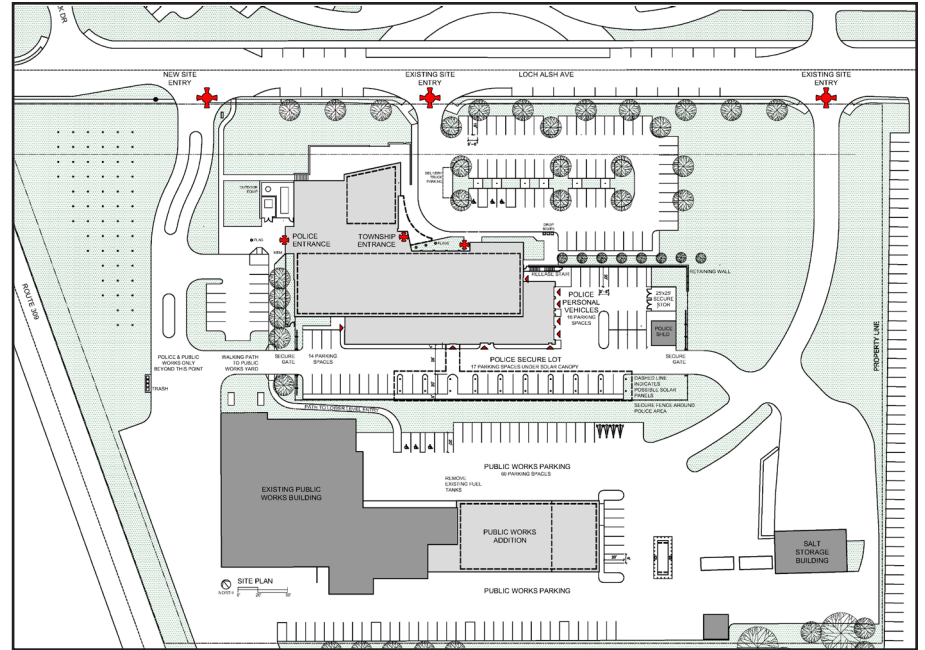
CONCEPT PLAN Proposed Township Building 52,016 Sq Ft
