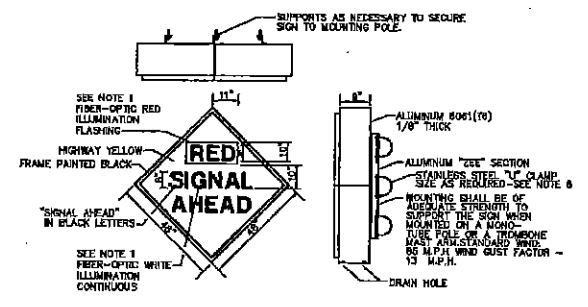
DETAIL "RED SIGNAL AHEAD" SIGN "V" MOUNTING ARRANGEMENTS NOT TO SCALE
